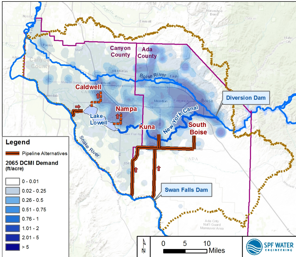
Figure 15. Conceptual Snake River conveyance alternatives.
